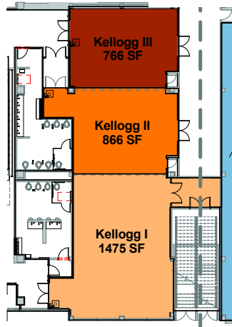
Lobby Level
